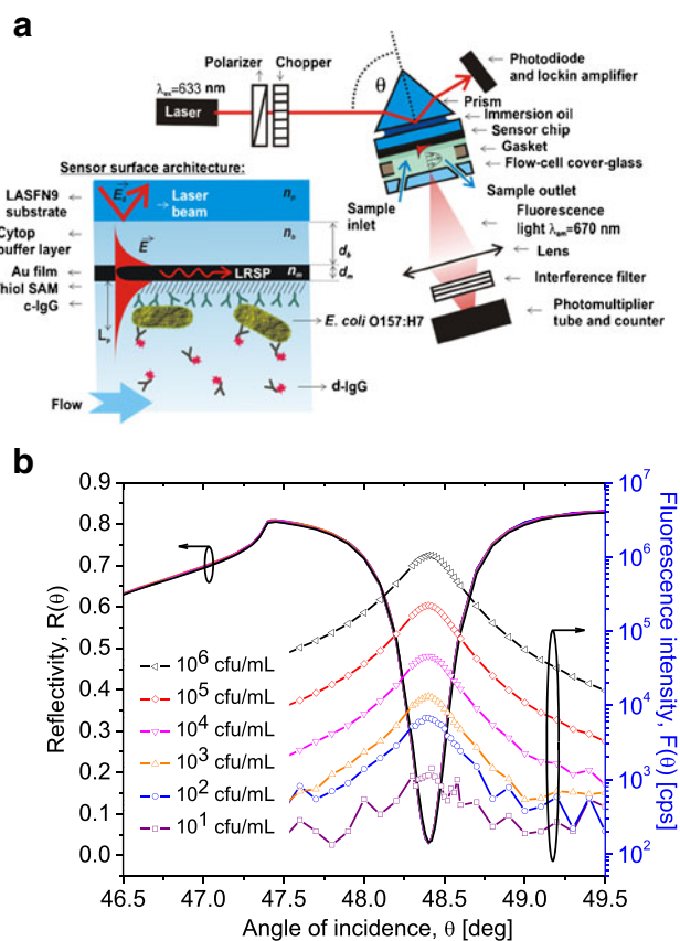
Fig. 9 a Optical setup of surface plasmon-enhanced fluorescence spectroscopy (SPFS) utilizing angular modulation of SPR. Example of a sensor chip supporting LRSPPs and E. coli O157:H7 sandwich immunoassay format. b Fluorescence signal measured upon the changing angle of incidence of the excitation laser beam in vicinity to the resonance after binding of target analyte ( E. coli O157:H7) and reacting with dye-labeled detection antibody on the surface (reproduced with permission from [119])
