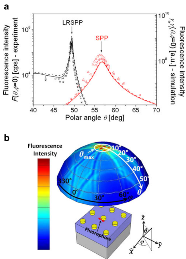
Fig. 3 a Simulated and experimental angular dependence of surface plasmon-coupled emission via regular surface plasmon polaritons (SPPs) and long-range surface plasmon polaritons (LRSPs) with reverse Kretschmann configuration. b Angular distribution of emitted light from a dipole coupled with arrays of metallic nanoparticles supporting collective localized surface plasmons (reproduced with permission from [65] and [53])
